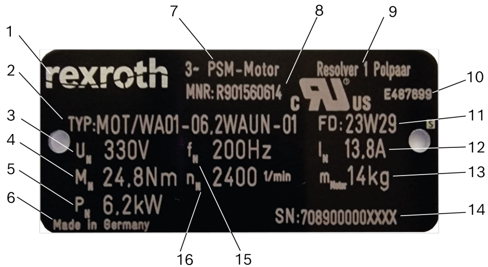
Fig. 3: Motor name plate
