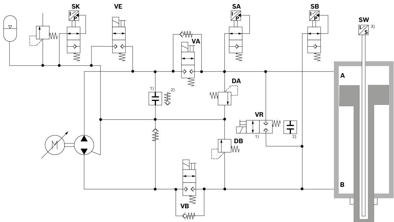
Fig. 9: Hydraulic circuit diagram
