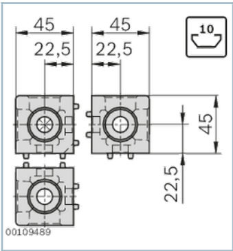
Central bolt S12x30-T50
