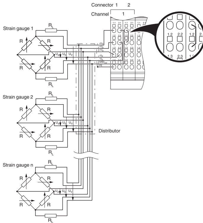
Fig. 5 Connection of several strain gauges in 6-wire technology
