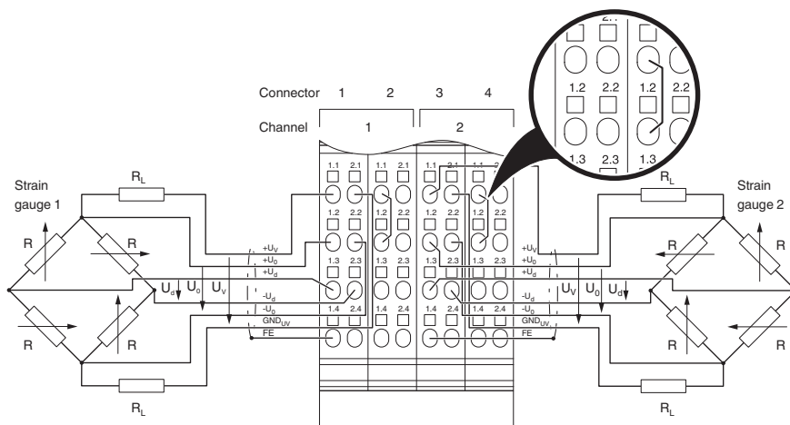
Fig. 4 Connection of strain gauges in 6-wire technology
