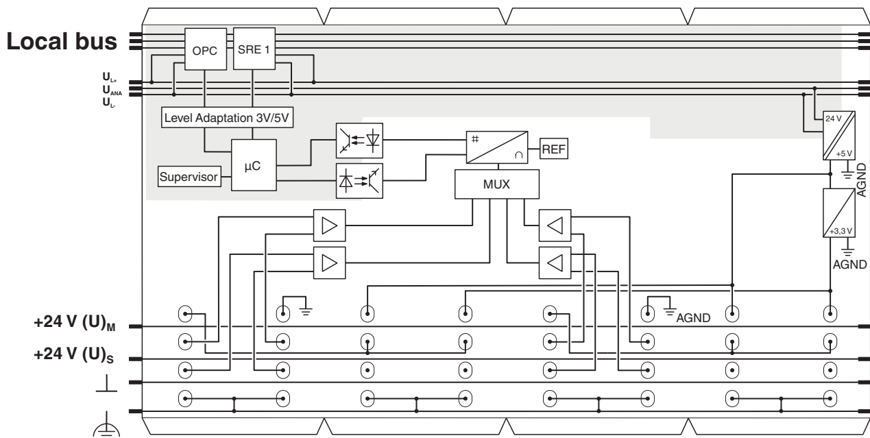
Fig. 1 Internal wiring of the terminal points
