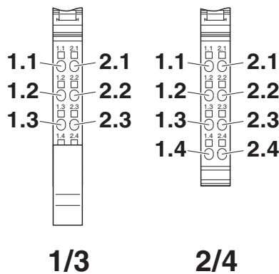
Fig. 2 Terminal point assignment
