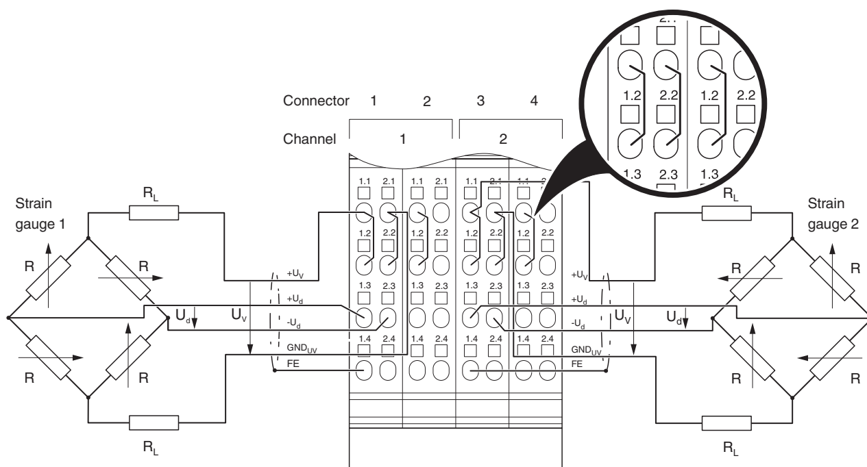
Fig. 6 Connection of strain gauges in 4-wire technology (channel 1 and channel 2)
