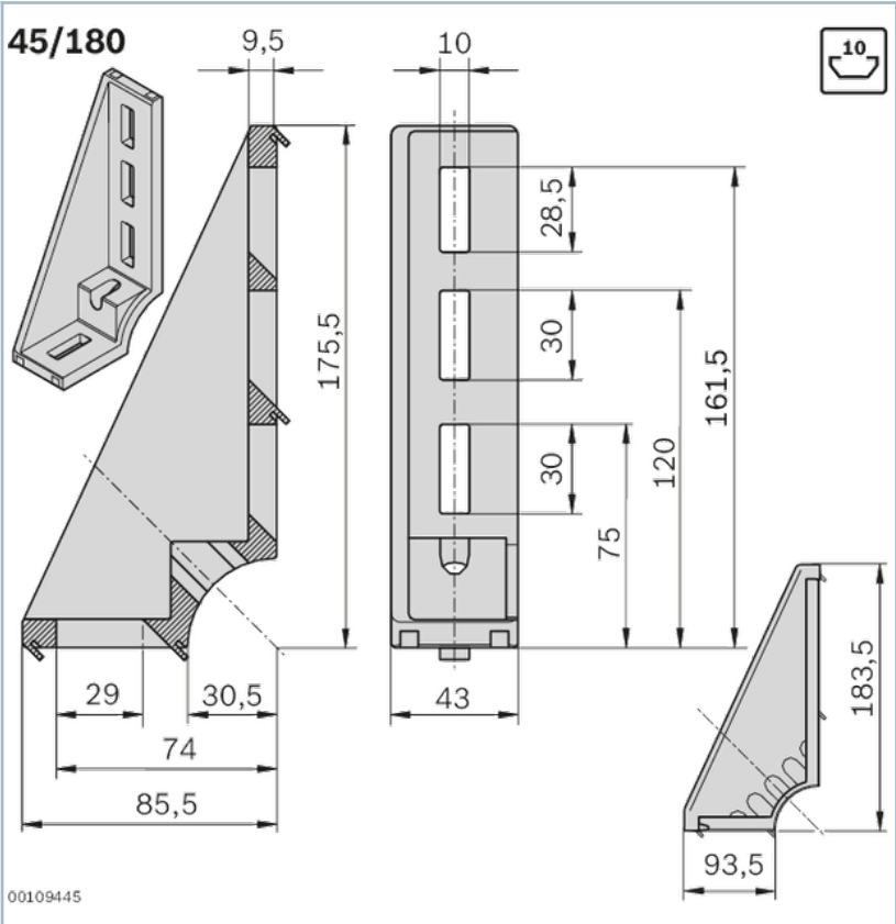
Bracket 45/180 with cover cap
