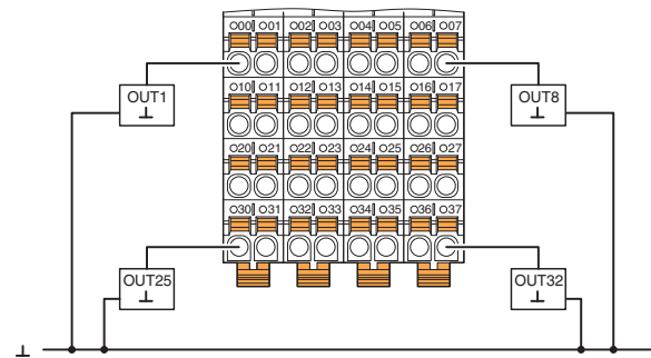
Fig. 5 Connection in 1-conductor technology
