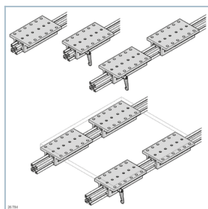
EcoSlide 45x45x80 sliding carriage
