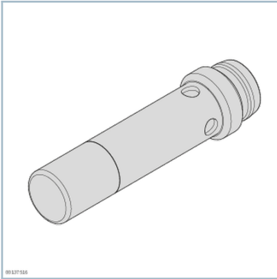
M12 sensor Ø 6.5 mm with M8x1 push-in fitting
