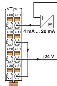
Differential current input with passive 2-conductor transmitter (current loop)
