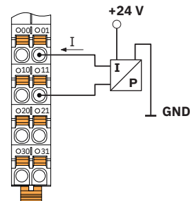
Active pressure sensor at a differential current input
