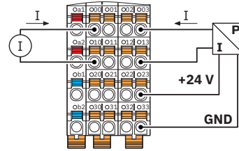
Fig. 3 Connection for current measurement
