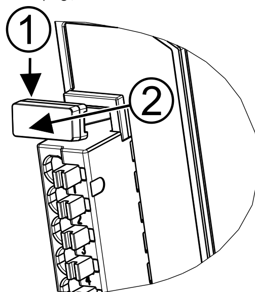
Fig. 6: Removing plug
