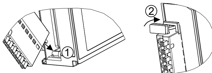
Fig. 5: Positioning plug
