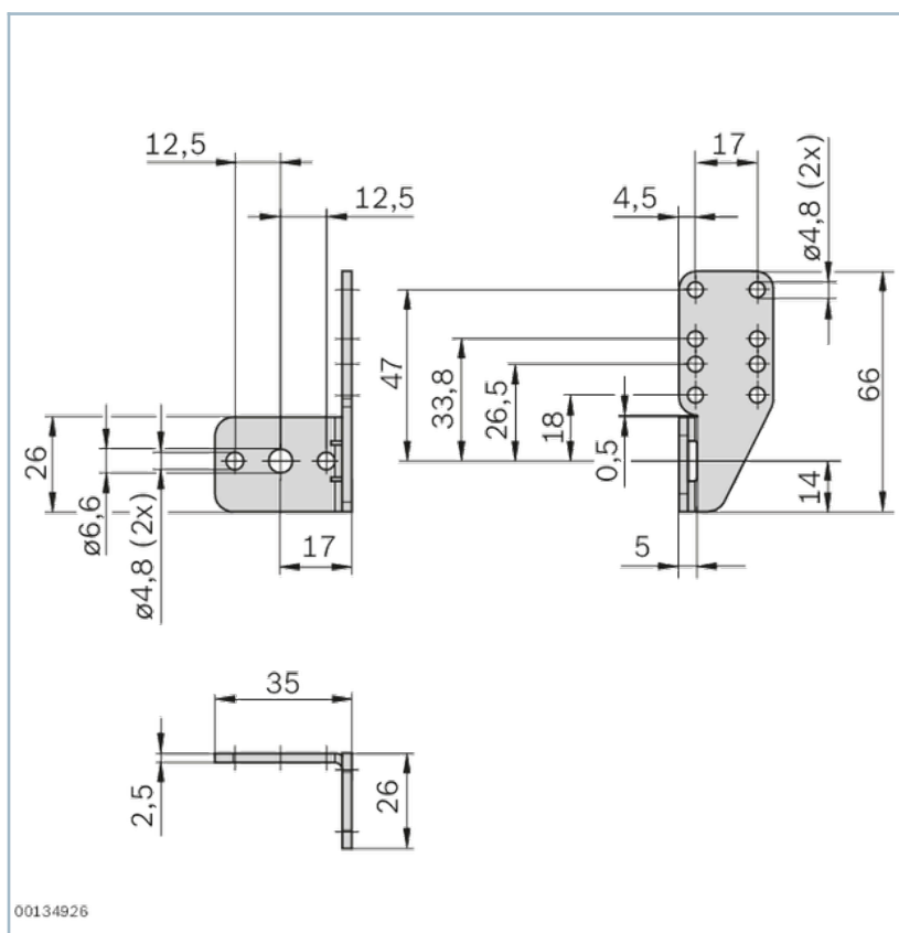
Fastening kit ID 15/MS-1
