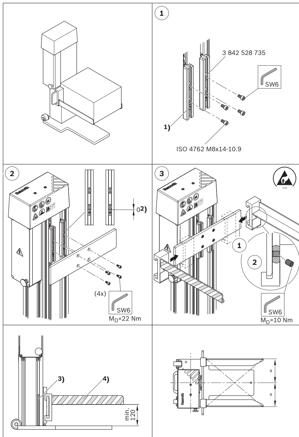
Fig. 7: Montering monteringsplate, gafler for kasser
