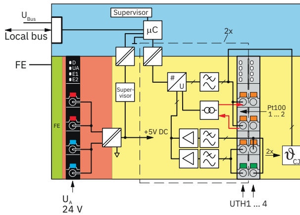
Fig. 4 Internal wiring of the terminal points
