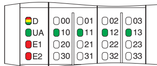
Fig. 14 Local diagnostic and status indicators
