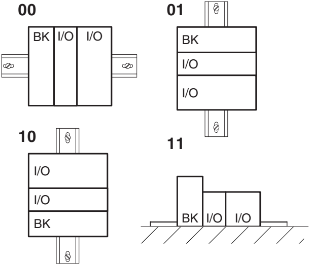
Fig. 15 Mounting position
