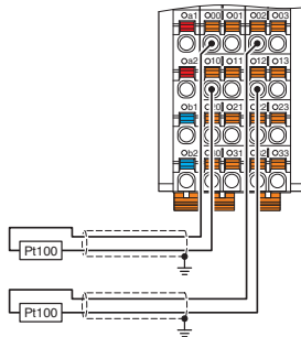
Fig. 11 Pt 100 detection
