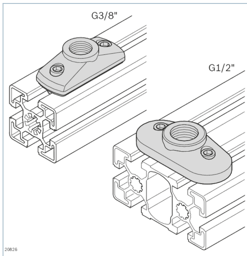
Air-supply elements
