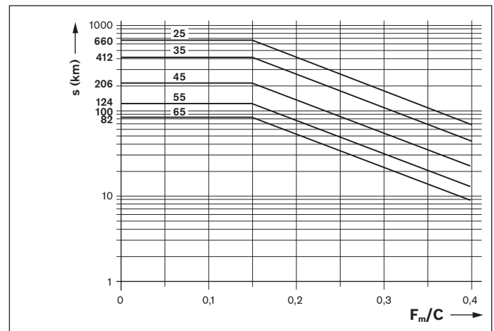
Fig. 2: Relubrication interval
