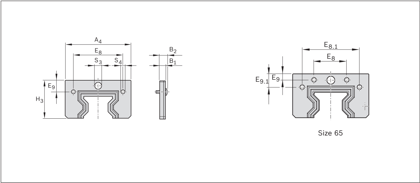
Material numbers and dimensions
