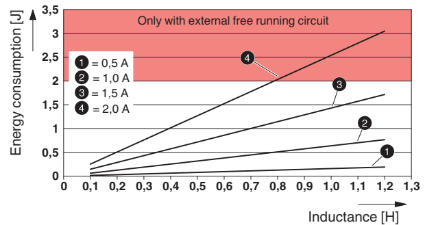
Fig. 3 Maximum energy consumption of the outputs when switching off inductive loads with 50 % simultaneity
