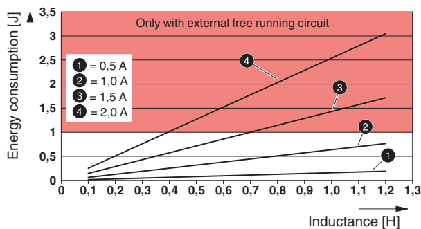
Fig. 2 Maximum energy consumption of the outputs when switching off inductive loads with 100 % simultaneity
