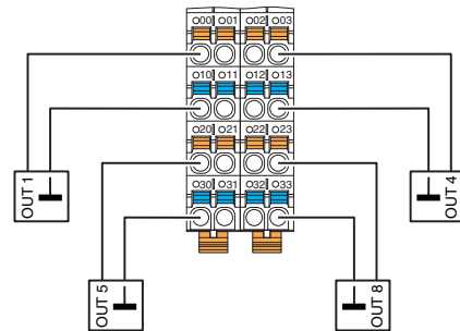
Fig. 7 Connection in 2-conductor technology
