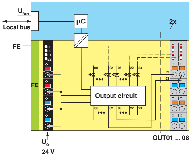
Fig. 4 Internal wiring of the terminal points
