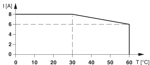
Fig. 1 Derating diagram for channel groups 1 ... 4 and 5 ... 8
