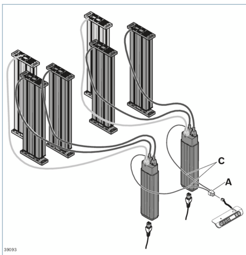
Synchronization of a maximum of 6 lifting columns with a maximum of 2 control units
