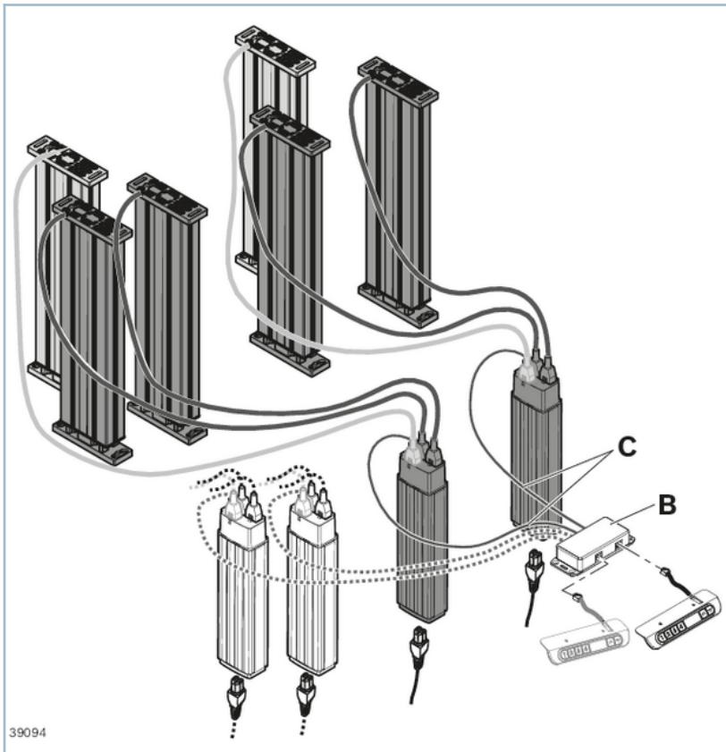
Synchronization of a maximum of 12 lifting columns with a maximum of 4 control units
