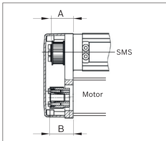
Fig. 13: Dimensions A/B
